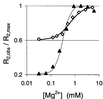
Figure 6. The effect of [\text{Mg}^{2+}] on MeOPH relaxation in solutions of RRE1 ( 20 \mu\text{M} ) in 25 \text{ mM K}^+ (filled triangles) or 100 \text{ mM K}^+ (open diamonds) and \text{Mn}^{2+} ( 3 \mu\text{M} ). Solid lines show behavior predicted by the K_d and n values in Table 1.
