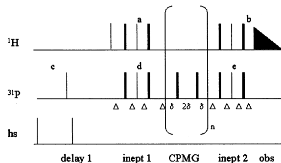
Figure 2. The one-dimensional pulse sequence for measuring phosphite 31 P T_2 values. Coherence originating on the phosphorus-bound proton ( 1 H–P) nucleus is transferred to the 31 P nucleus using a series of inept pulses. After a series of CPMG 180° refocusing pulses ( 31 P frequency), the remaining signal is returned to the 1 H–P nucleus for detection using a second series of inept pulses. The transverse relaxation times ( T_2 ) were determined from the slopes of the linear plots of \log(i) versus t , where i is the maximum intensity of the resonance and t is the time between the two inept series of pulses ( t = 4nd ). Narrow and broad lines represent 90° and 180° pulses on the indicated channel. A 90° 31 P pulse and two homospoil pulses are inserted into delay 1 to remove artifacts arising from residual magnetization remaining between transients. All pulse phases are zero unless noted otherwise. Delays in the inept 1 and inept 2 portion of the sequence ( \Delta ) are equal to 1/4J . The delay between CPMG pulses ( \delta ) was 4 ms. The T_2 delay was varied by changing the number of times through the CPMG cycle ( n ). Phase cycles were as follows: a = (1,1,1,1,3,3,3,3), b = (2), c = (3,3,3,3,3,3,3,3,1,1,1,1,1,1,1,1), d = (0,2), e = (0,0,2,2), and obs = (2,0,0,2,0,2,2,0).
