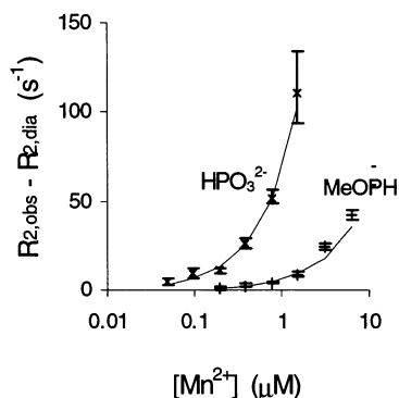
Figure 3. Semilog plot showing the effects of [Mn^{2+}] on ^{31}P transverse relaxation rates ( R_{2,obs} ) of phosphite dianion ( HPO_3^{2-} , represented by the X within the error bars) and methyl phosphite anion ( CH_3OP(H)O_2^- , represented by a +), corrected for diamagnetic relaxation rate ( R_{2,dia} ). R_2 of HPO_3^{2-} is a factor of 10 more sensitive to [Mn^{2+}] than the R_2 of MeOPH. Lines show behavior predicted for relaxation enhancement proportional to [Mn^{2+}] .
