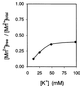
Figure 5. The effect of [K^+] on free Mn^{2+} in solutions of A-site (27 \mu M ) and Mn^{2+} (16 \mu M ), as determined from R_2 data (Figure 3).
