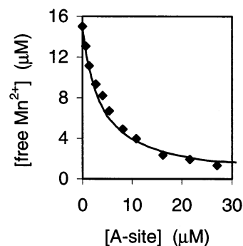
Figure 4. The effect of A-site RNA on free Mn^{2+} (5 mM PIPES, pH 7.2, 5 mM MeOPH, K^+ salts). The line represents behavior predicted for seven independent binding sites having K_{d,Mn} = 25 \mu M .
