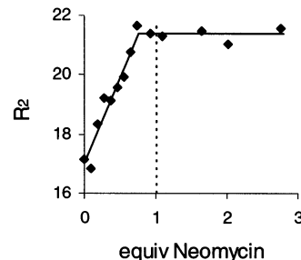
Figure 7. The effect of neomycin b on the relaxation rate ( R_2 ) of the \text{HPO}_3^{2-} \text{ } ^{31}\text{P} signal in solutions of A-site RNA ( 2.7 \mu\text{M} ), \text{Mn}^{2+} ( 0.11 \mu\text{M} ), and 100 \text{ mM K}^+ .
